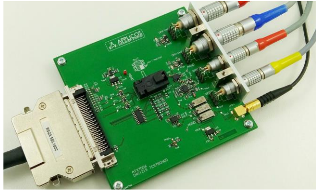
Test fixture with 5 analog signal connections and a DIO connection.
