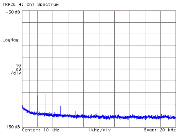
DC to 20kHz spectrum, 1KHz carrier, 96ksps, 22kHz filter (levels are dBc, carrier above 50dB not shown).
